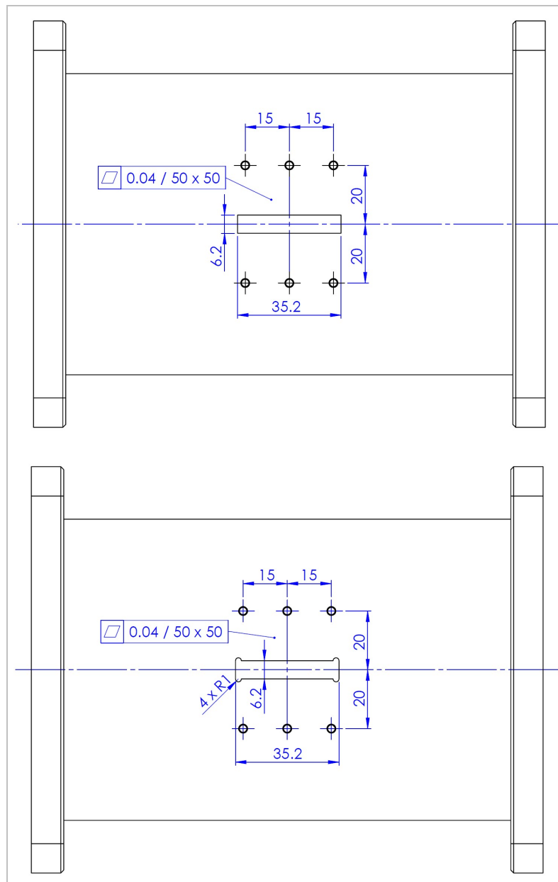
Fig. 4. Waveguide machining templates. All dimensions are in millimeters. The waveguide dimensions are not to scale. The bottom alternative is for a better manufacturability. The waveguide wall thickness must be 2 mm. Suggested are M3 x 8 screws (stainless or galvanized steel).
