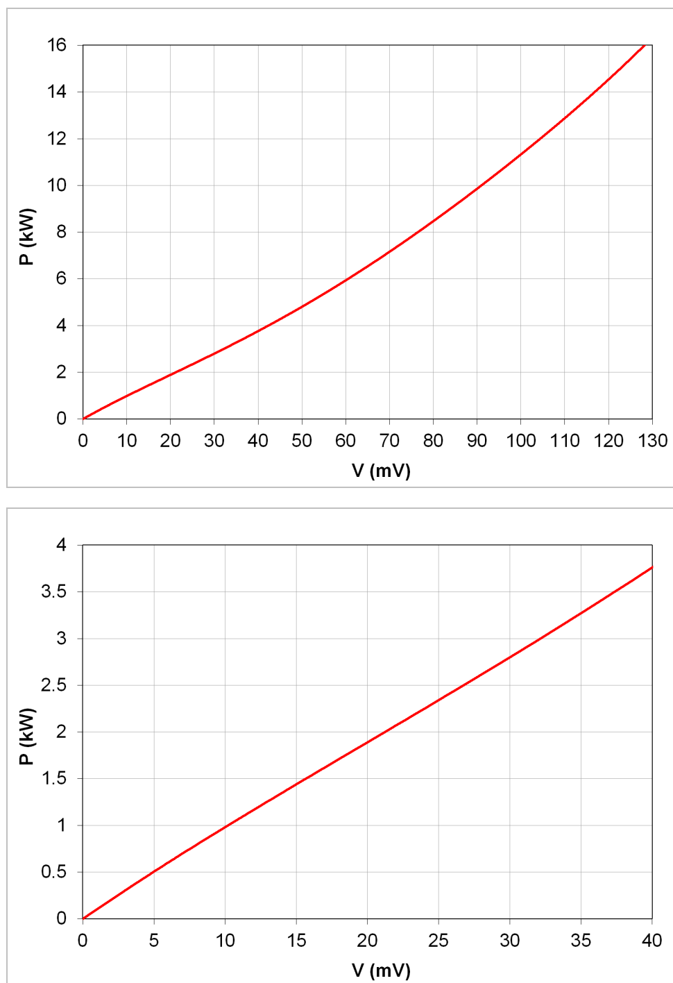
Fig. 2. Typical DD131 correction curve.
