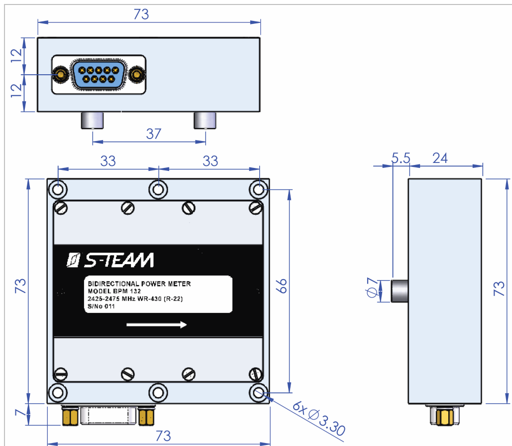
Fig. 13. Basic BPM132 dimensions in millimeters.
