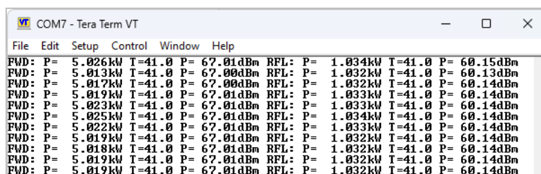
Fig. 8. Example of RS232 digital output.
